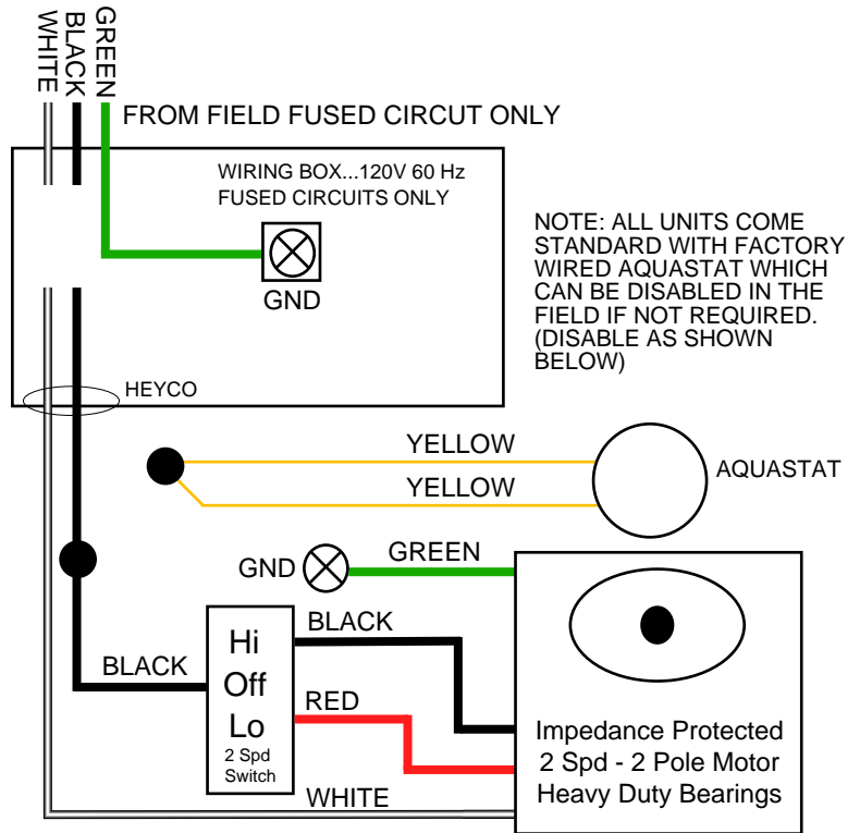
KWM 4+, 6+ AND KWM 11+ WIRING WITH AQUASTAT DISABLED
