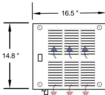
DOUBLE DOWN COVER COVER VIEW
