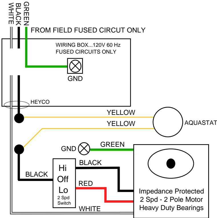
KWM 4+, 6+ AND KWM 11+ STANDARD WIRING DIAGRAM
